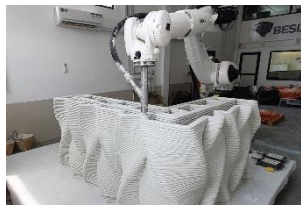
Beton 3D-Druck
